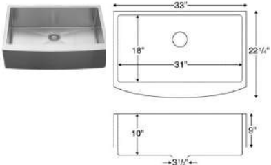
EL-84 33" x 22-1/4" (outside dim.) Single Bowl Under-mount Karran 16 Gauge Stainless Steel Apron Sink (min. 36" apron sink base cabinet)
